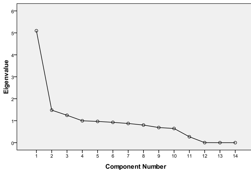
Figure 7-2 Scree Plot
