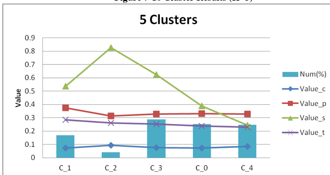
Figure 7-10 Cluster Results (K=5)
